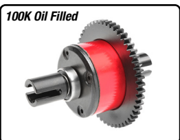
C-00180-685-1 Centre Diff Assembly - Alu / Steel - 52T Main Gear - 1 set
